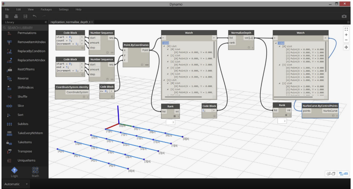
Figure 14 In Dynamo , in order to correct for the side effect [in Figure 13] the user has to add a 'work around', which is to 'normalise the depth' of the point array. But this introduces an addition concept 'normalise depth' for the novice user. Having to understand this additional concept might become an 'abstraction barrier' for some novice users
