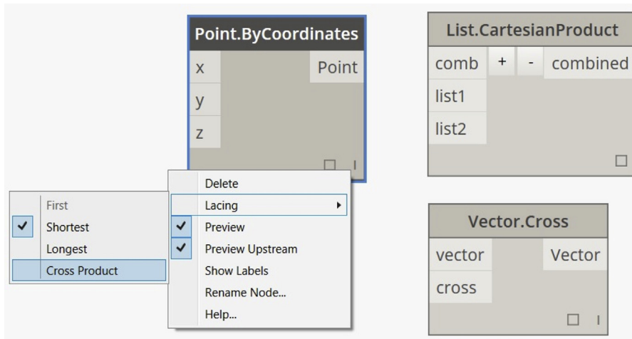
Figure 12 In Dynamo to create the 2D array of points, the user needs to combine the sequence of X coordinates with the sequence of Y coordinates using the 'Cross Product' option. [See 'Semantic Interference' section]
