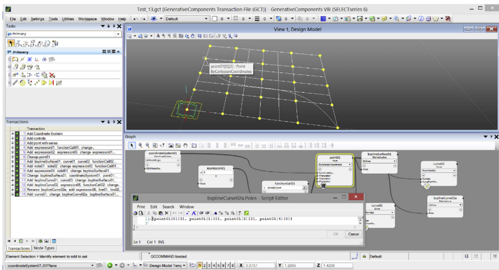
Figure 4 The ‘S’ curve was create by selecting points from the point array directly in the geometry window. Note the identity of the point selected is displayed as part of the flyover label with the indexing into the 2D point array. The corresponding graph node is highlighted. The collection expression code fragment [in the script editor] is being built for the user from the interaction with the geometry model. As the user selects a further point so the collection expression is automatically extended with a new member
