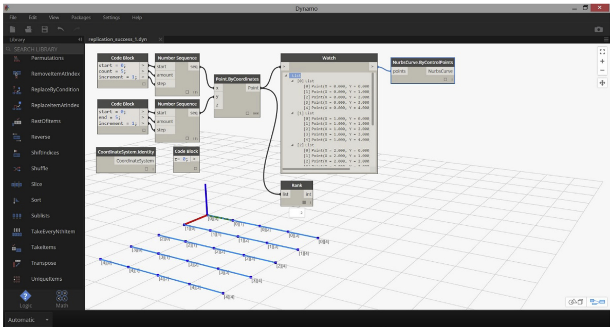
Figure 10 Creating a 2D point collection. This uses a sequence of X coordinates and a sequence of Y coordinates and the default value [0.0] for Z. This 2D point collection can directly be used to create the collection of curves, or a surface [not shown]. Note: the Z coordinate is not defined and the default value of zero is used
