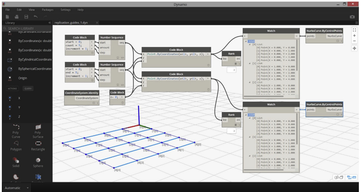
Figure 16 An alternative way to create the array of points is to use a code block node and a DesignScript expression with the underlying 'Point.ByCoordinates method using replication guides <1> and <2> to control the replication behaviour
