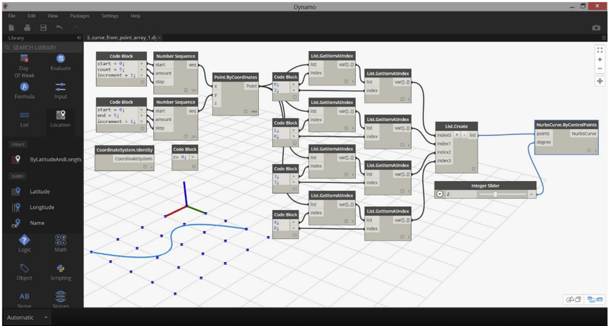
Figure 18 In Dynamo using the available nodes, to select points to create the 'S' curve, the user has to repeat a complex two stage selection process, first selecting the sub list from the 2D collection and then selecting the specific point from the sub list. There is no multi-index [or path] selection node to select an item from a multi-dimensional collection. 13 nodes are required to select 4 points
